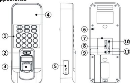
Figure 1. 1 Appearance of DS-K1T803 Series model Table 1. 1 Description of DS-K1T803 Series Model
